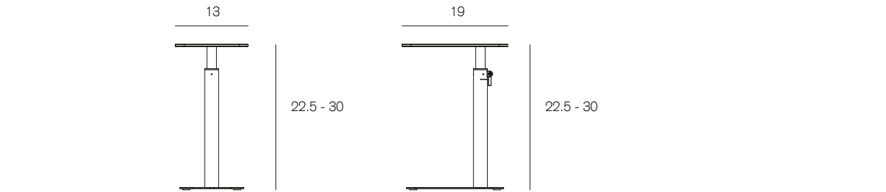
Height adjustable
